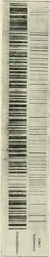
FIG. 22.—Comparison of the spectrum of the chromo-sphere with the test-spectrum.
